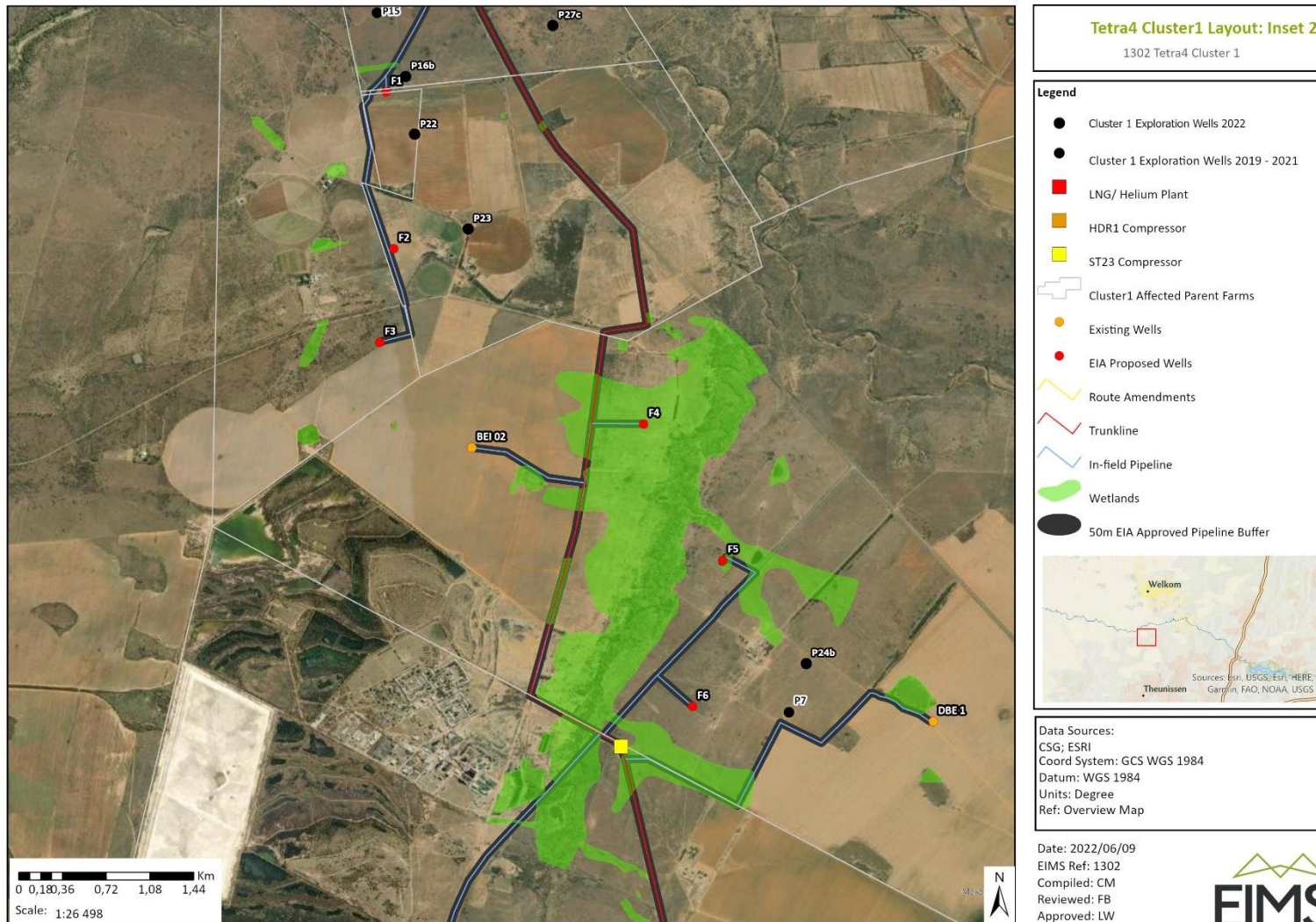
Figure 3: Layout Map of the Cluster 1 Gas Production Project area (Inset 2). 3
