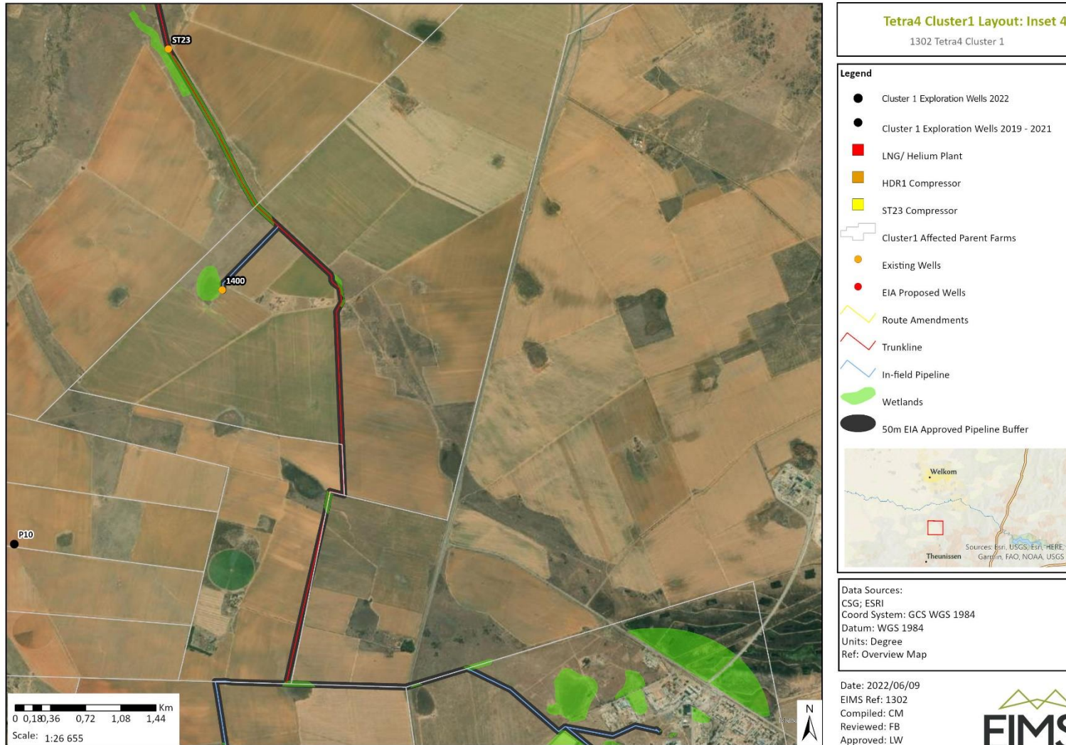
Figure 5: Layout Map of the Cluster 1 Gas Production Project area (Inset 4). 4
