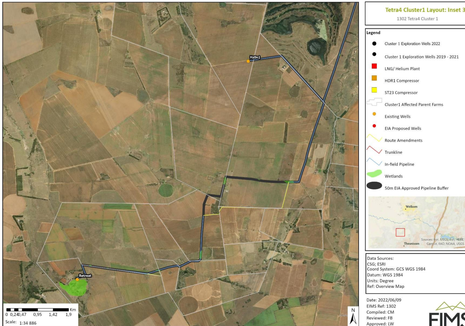
Figure 4: Layout Map of the Cluster 1 Gas Production Project area (Inset 3).
