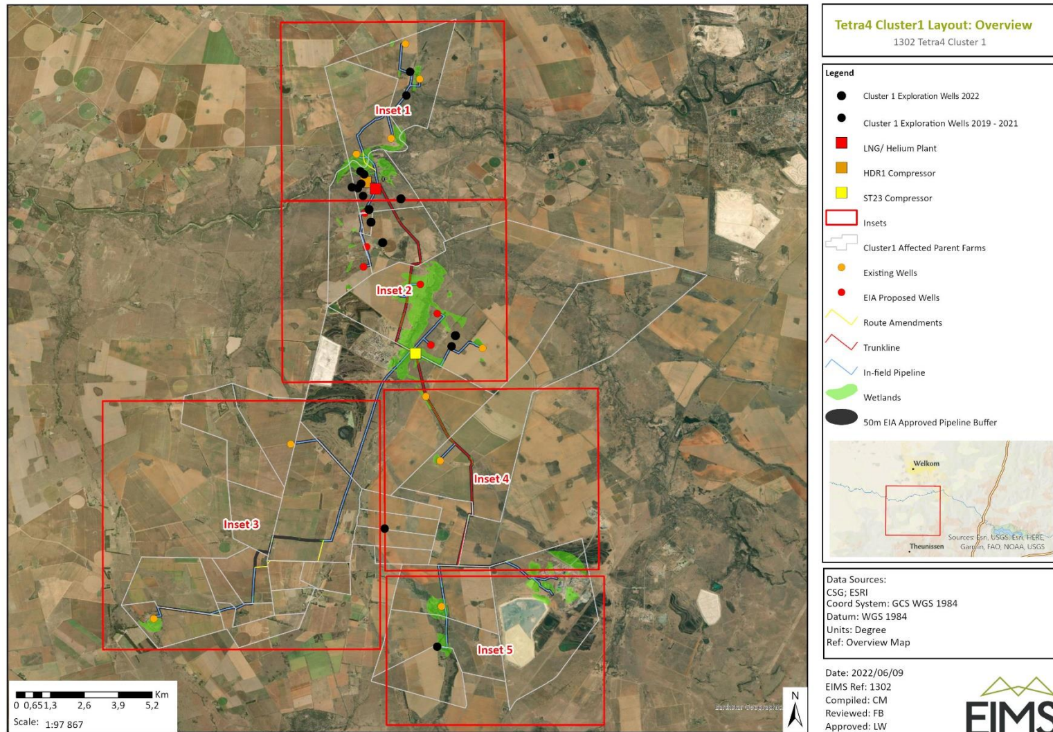
Figure 1: Layout Map of the Cluster 1 Gas Production Project area (Overview) 1 .
