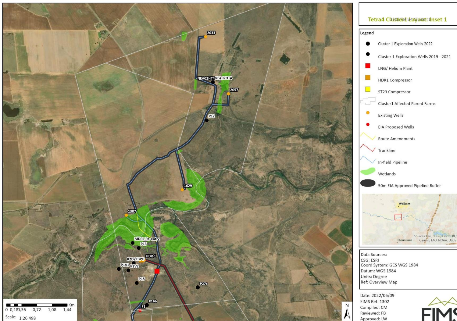
Figure 2: Layout Map of the Cluster 1 Gas Production Project area (Inset 1) 2 .
